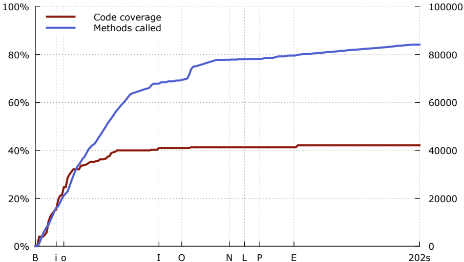
Code coverage breakdown for Obad
